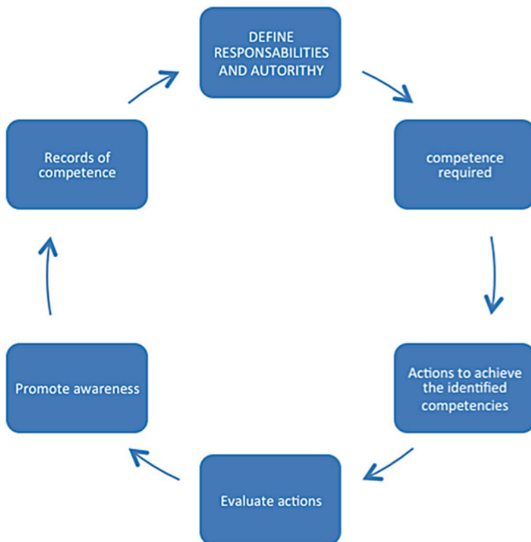
Fig. 8.2 Guidelines about HR in ISO 9001. Source: authors
